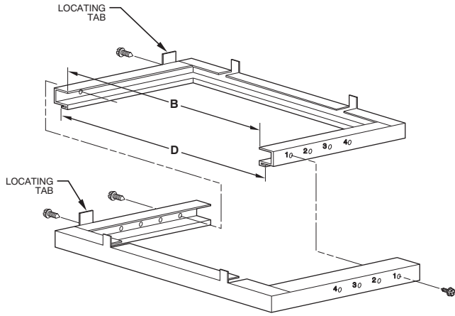
Disassembled
